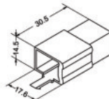
XJY09001G-3Y ZC09
