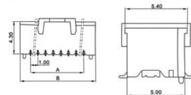
•XJ1001J-NA
