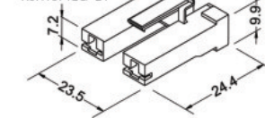
XJR18712G-2Y
