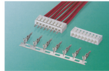
• XJSAN00-B
