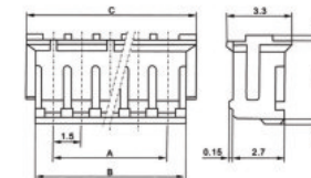
•XJ1500J-A(ZH)
