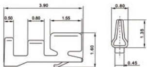
•XJ1001J-NY
