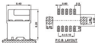
•XJ1001J-NA
