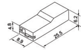
XJR25012G-1Y
