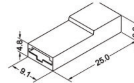
XJR25011G-1Y
