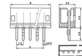
•XJ1500J-A(ZH)
