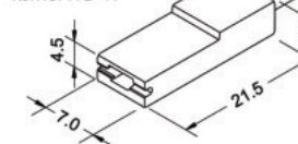
XJR18711G-1Y
