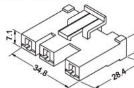
XJR18712G-3Y
